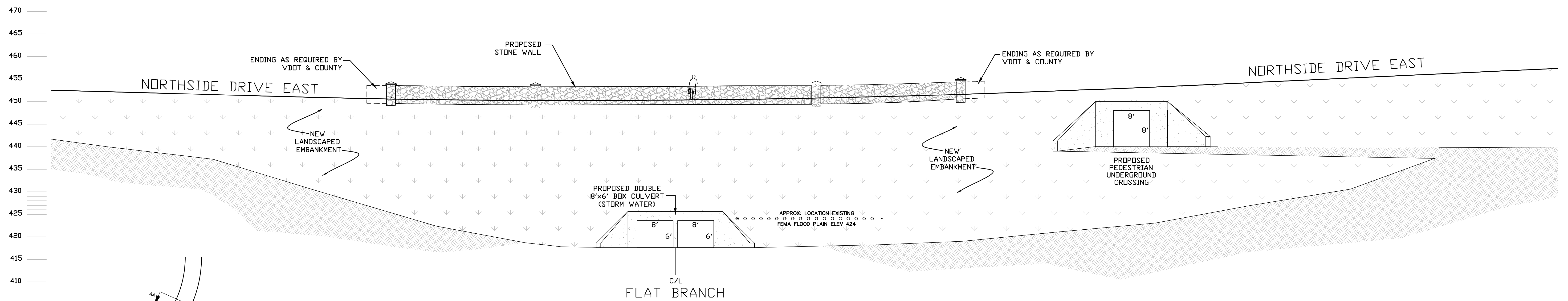
NORTHSIDE DRIVE STREAM CROSS-SECTION BB (LOOKING NORTH)
